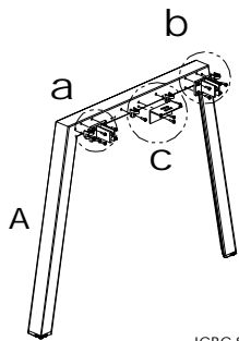
JCBC Screw M6x35
